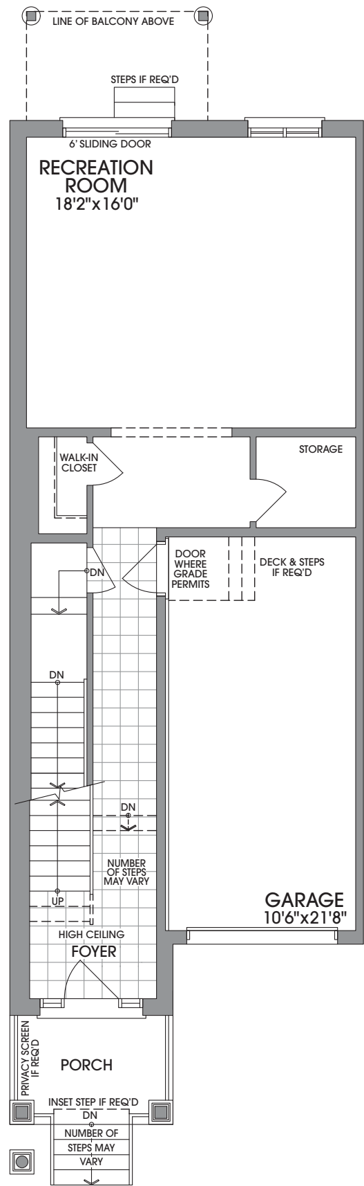
GROUND LEVEL Elevation A
