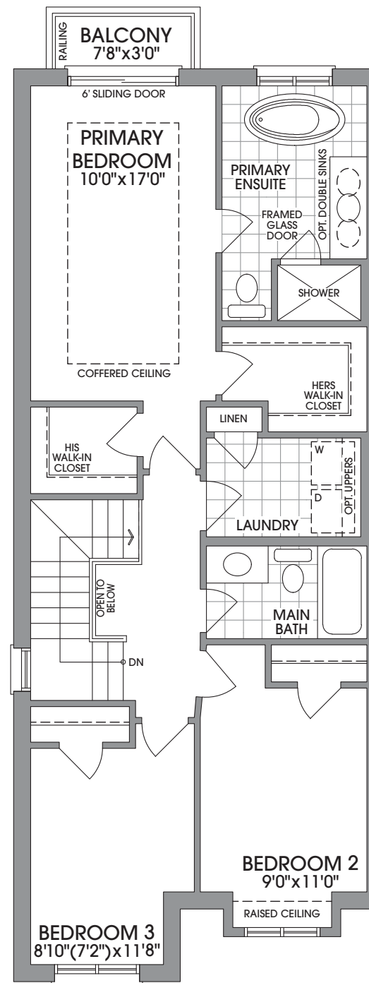
UPPER LEVEL Elevation A
